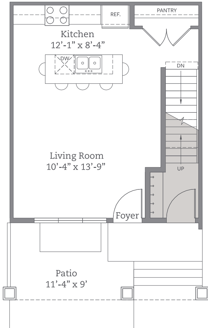
Main Floor 425 Sq.Ft.
