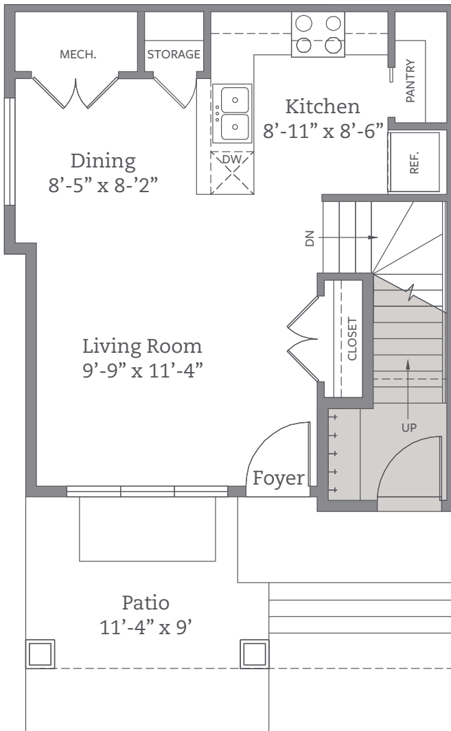
Main Floor 442 Sq.Ft.
